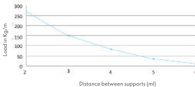
Load curve ECC4
